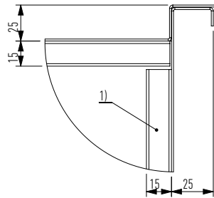
DETAIL B SCALE 1 : 3
